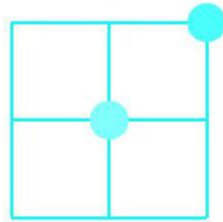
D_4 Lattice
