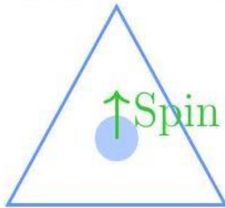
D_3 Gyroscope
